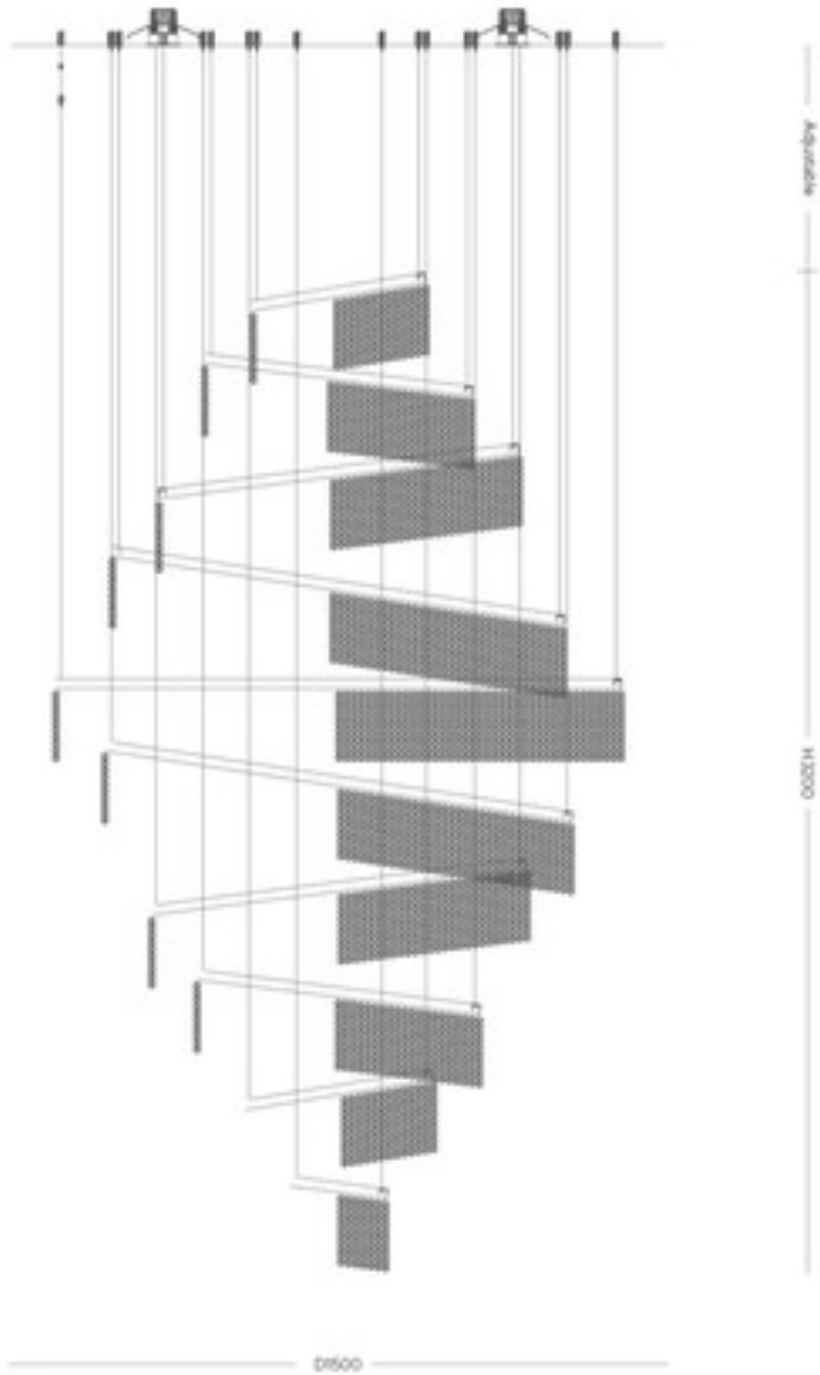
9268-1500(10 ring) Size: D1500*H3200mm
